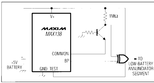
Figure 6. Low-Battery Detector and LCD Segment Drive
